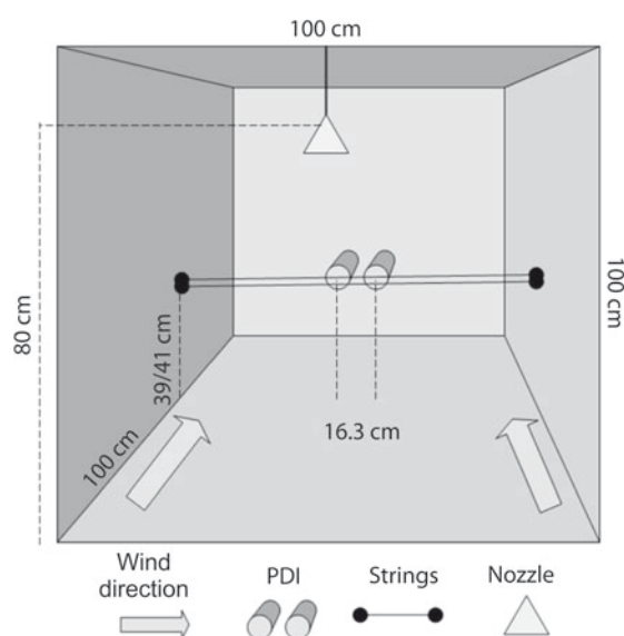
Fig. 1. Schematic of tunnel set up
