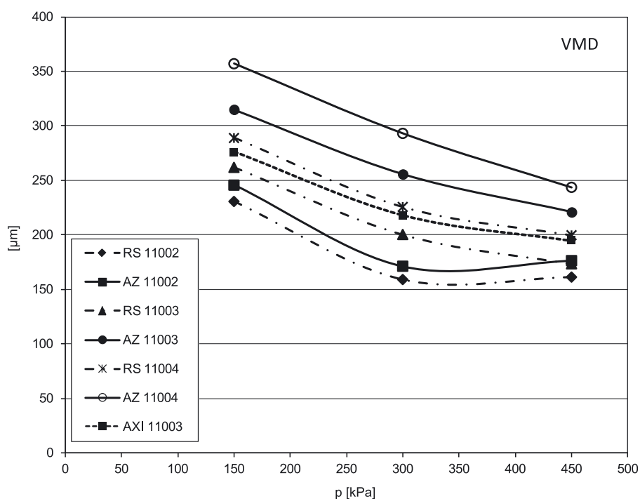
Fig. 2. Droplet size characteristics for tested nozzles interpreted with VMD
