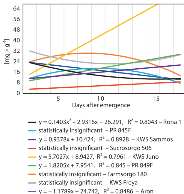
Fig. 2. The sorgoleone content in the dry matter of sorghum roots; HSD 0.05 (5 DAE) = 1.13; (10 DAE) = 1.39; (15 DAE) = 1.33; DAE – days after emergence
