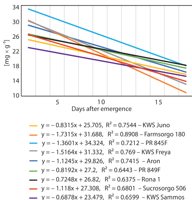
Fig. 1. The phenolic acid content in the dry matter of the above-ground parts of sorghum; HSD 0.05 (5 DAE) = 6.84; (10 DAE) = 5.37; (15 DAE) = 1.98; DAE – days after emergence
