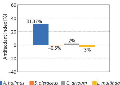
Fig. 3 Antifeedant effects of four different medicinal plant extracts against Tribolium castaneum adults
