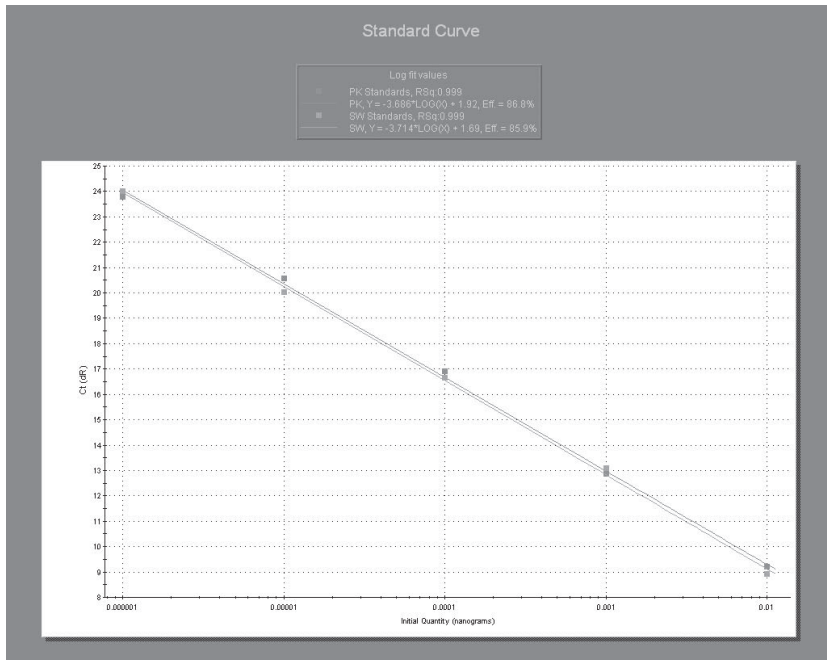
Fig. 3. Standard curves prepared with the primers F5 and R5 and 10-fold serial dilutions of PepMV-PK and PepMV-SW total RNA
