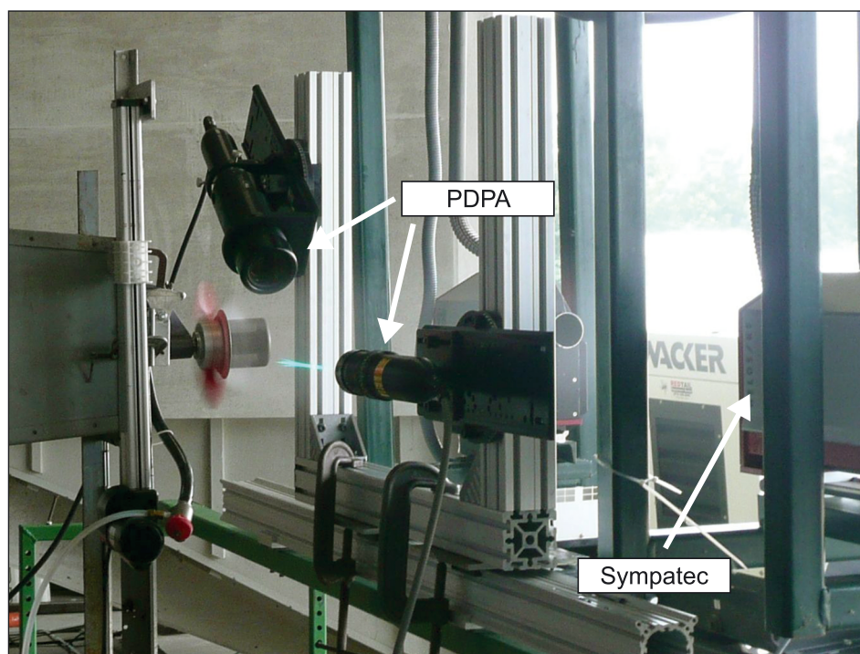
Fig. 3. Phase Doppler Particle Analyzer (PDPA) and Sympatec HELOS particle size measurement systems positioned at the exit of the high speed wind tunnel (HSWT)
