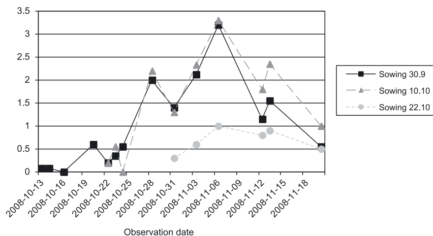
Fig. 6. Density dynamics of O. florum (flies/m²) in relation to sowing date, 2008, Kostinbrod
