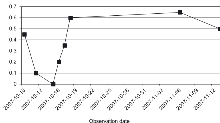
Fig. 5. Density dynamics of O. florum (flies/m²) in relation to sowing date, 2007, Kostinbrod
