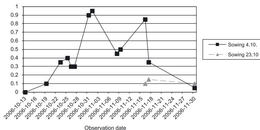
Fig. 4. Density dynamics of O. florum (flies/m²) in relation to sowing date, 2006, Kostinbrod
