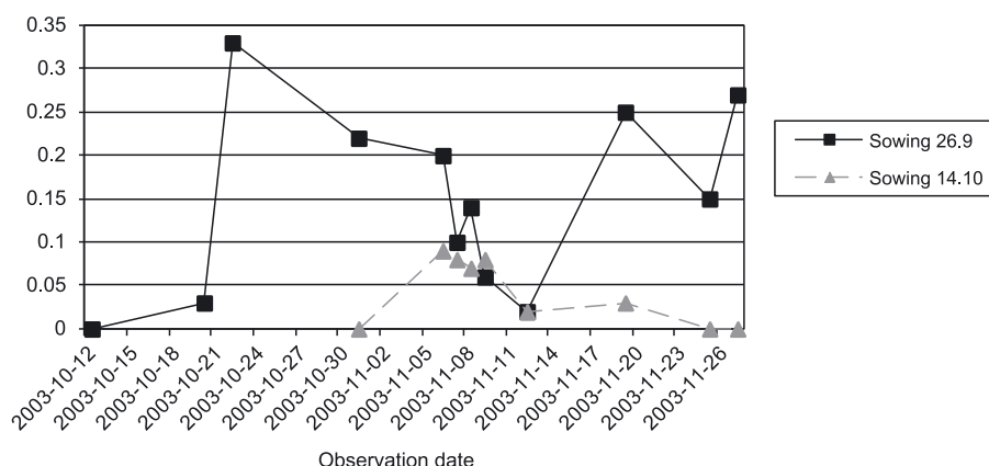
Fig. 1. Density dynamics of O. florum (flies/m²) in relation to sowing date, 2003, Kostinbrod
