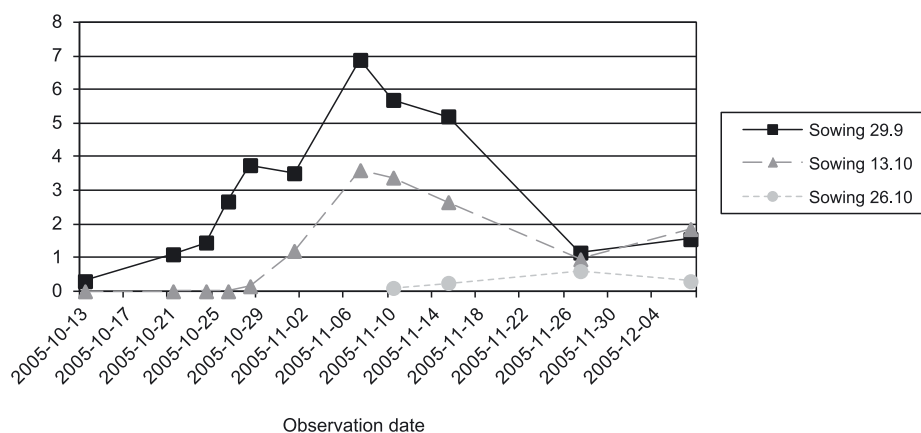
Fig. 3. Density dynamics of O. florum (flies/m²) in relation to sowing date, 2005, Kostinbrod
