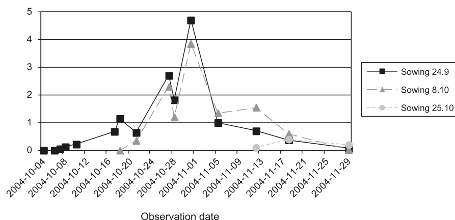
Fig. 2. Density dynamics of O. florum (flies/m²) in relation to sowing date, 2004, Kostinbrod
